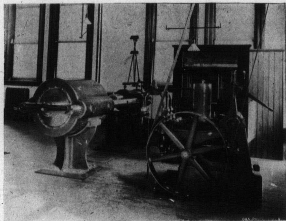
EMERY TESTING MACHINE.
