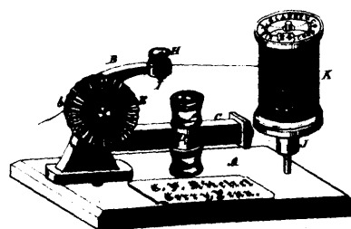
5852 Ritchel's Improvements in Sewing Machines.
