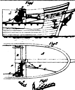
5853 Galliac's Improvement on Anchor Trippers.
