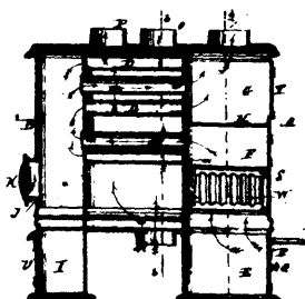
5851 Ruttan's Improvements in Heating Stoves.
