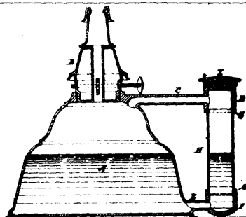
5848 Sedgwick's Devices for filling Lamps and other Vessels, and indicating the Height of Liquid in the same.
