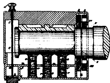
6095 Beattie's Improvements on Axle Boxes.
