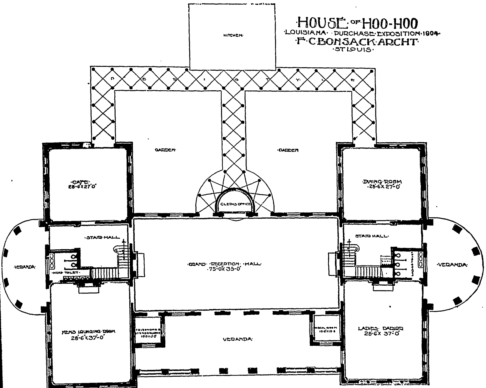
FIRST FLOOR, HOUSE OF HOO-HOO.
