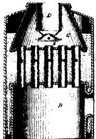
10012 Kratz's Improvements in Steam Boilers.
