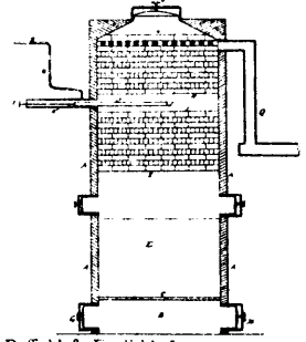
14851 Duffield & English's Improvements in the Processes and Apparatus for Manufacturing Gas.
