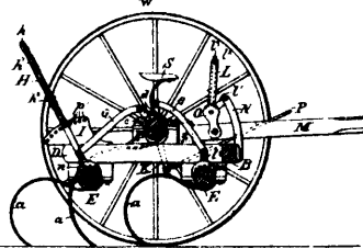
14854 Springer & Ives's Improvements on Spring Tooth Harrows or Cultivators.
