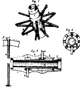
14850 Smith's Improvements on Wheel Hubs.
