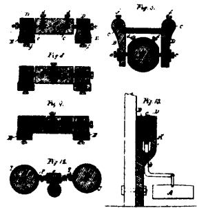
14855 Improvements in Self-Levelling Ship's Berths.
