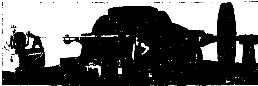
Represents a pair of 30-inch McCormick Turbines, with Governor and Fly-Wheel for regulating speed. The Turbine Shaft is direct connected to a 75 K. W. Generator.
