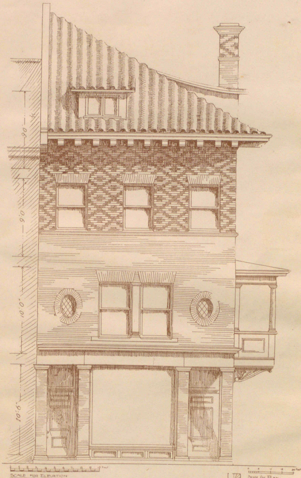
• FRONT ELEVATION •
