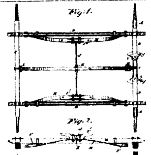
12003 Webster's Improvements on Carriage Springs.
