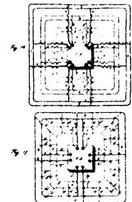
11997 Edison's Systems of Conductors for the Distribution of Electricity as a Lighting and Motive Power Agent.
