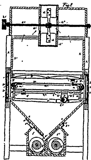
22714 Ponder's Middlings Purifier.
