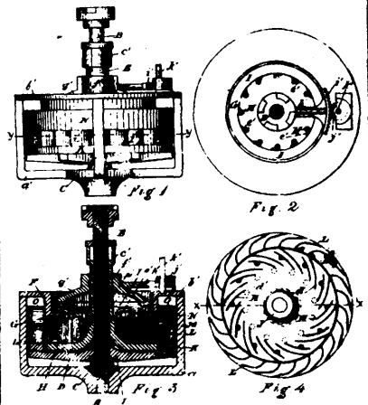
26904 Patrick's Water Wheel.
