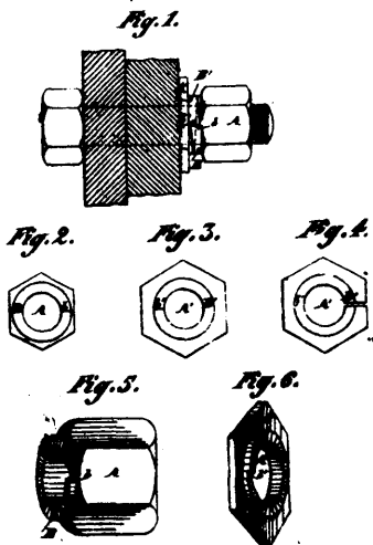
26908 Flamsche & Picard's Nut Lock.
