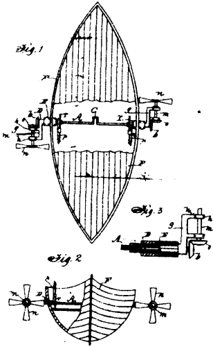
27518 Baker's Mechanism for Propelling Vessels
