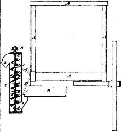
27515 Macpherson's Thrasher and Separator
