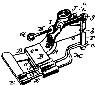
18570 Seckett's Ruffie Attachment for Sewing Machines.
