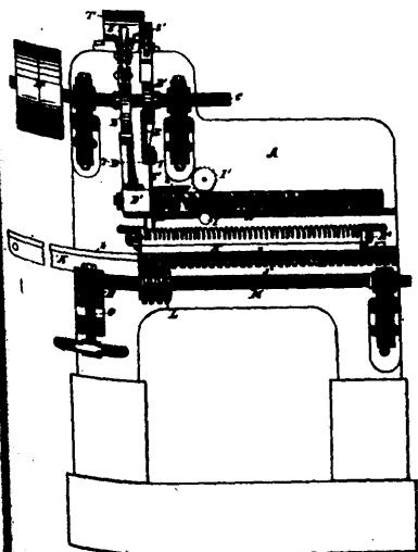
18569 Martin's Match Splint Machine.
