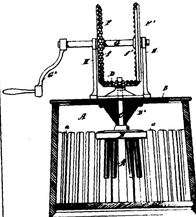
18567 Geneste's Washing Machine.
