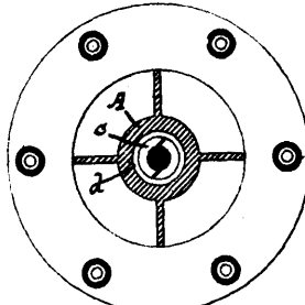
18573 Player's Metallic Packing for Piston Rods and Valve Stems in Stuffing Boxes.
