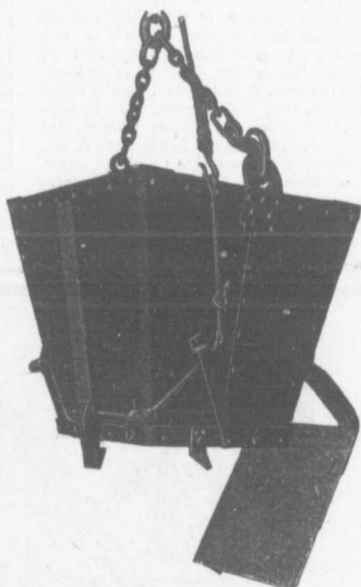
Bucket With Rope Tripping Device (Open)
