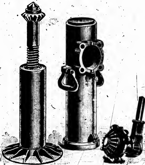
This Cut shows construction of Carpenters' and Builders' Jacks and Railway Jacks without Ball-bearing.
