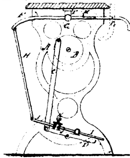
12416 Morton's Improvements on Sewing Machine Motors.
