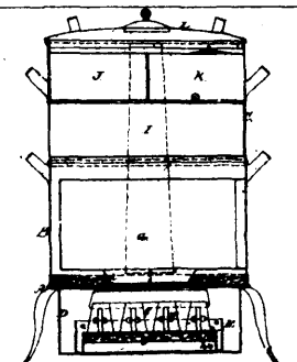
2533 Boyd's Steam Cooking Stove.
