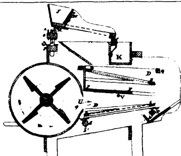
2524 Wood's Machine for Cleaning, Separating and Grading Grains, &amp;c.
