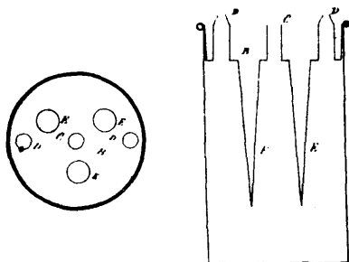
2521 Cass' Ventilating and Cooling Milk Can.
