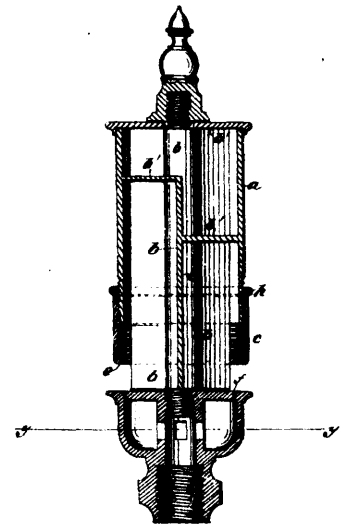
20266 Einig's Steam Whistle.
