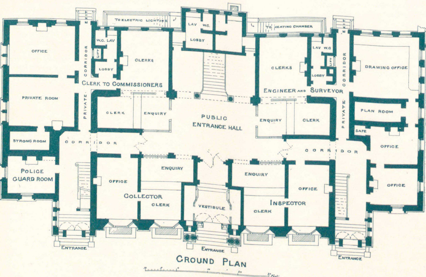
DESIGN FOR TOWN HALL. EDWARD SWALES, ARCHITECT.
