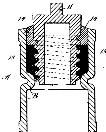
34540 Rossman's Plug for Pipes.
