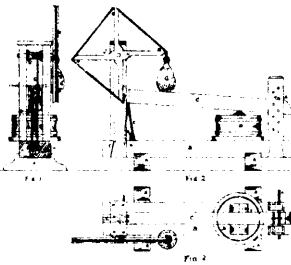
9557 Haylen's Improvements on Cheese Presses.
