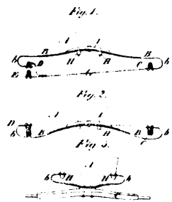
9569 Schultz's Improvements on Spring Carriages.
