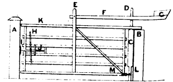
9563 Carpenter &amp; Walrath's Improvement on Farm Gates.
