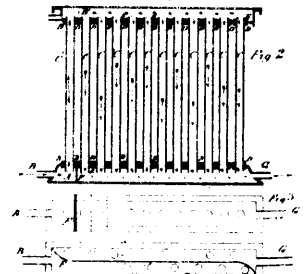
9558 McPhie's Improvements in Hot Water Radiators.
