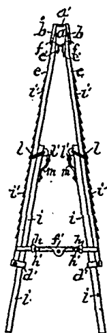
23674 Hooper's Adjustable Trestle.
