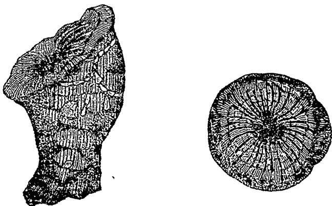
Fig. 18. Strombodes simplex , (Hall.)
