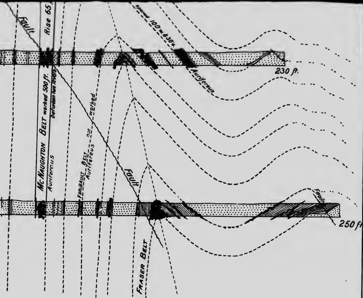
VERSE VERTICAL SECTION Main Shaft and Cross-cuts NOSE GOLD MINE, NORVILLE, NOVA SCOTIA.
