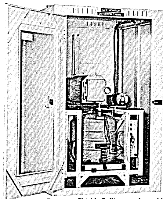
Detector/Shield/Collimator Assembly
