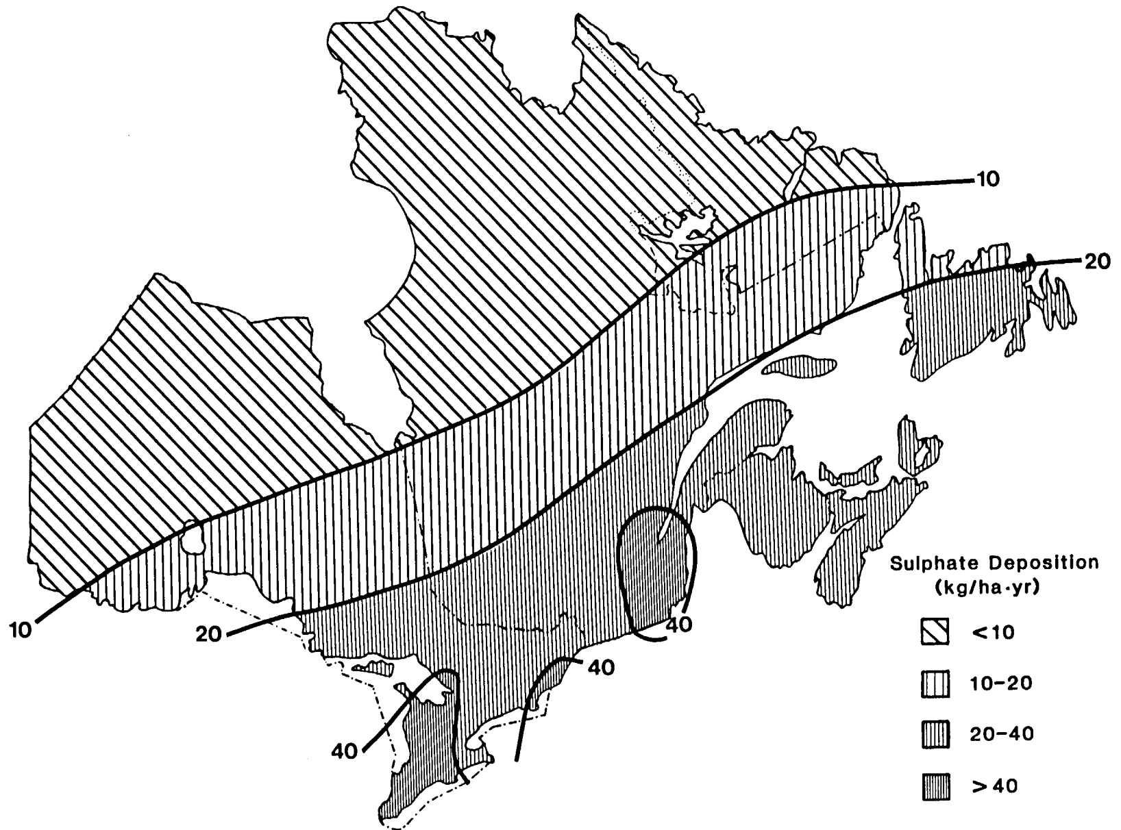
Figure 8-1b. Annual sulphate deposition regime for eastern Canada based on CANSAP 1980 data.
