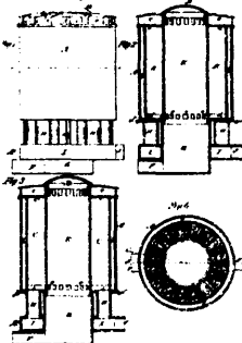
4165 Wilson's Furnace for Reducing Iron Ores.
