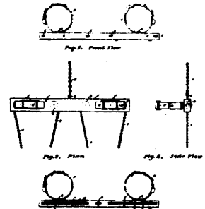
4167 White's Suspended Whiffletree.
