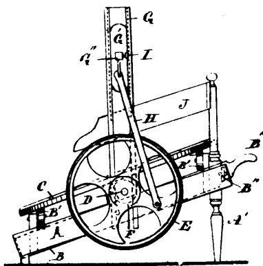
30829 Hamlin's Dog Power.
