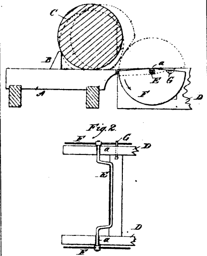
Park's Log Turner.
