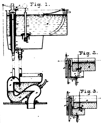
Boyle's Flushing Apparatus for Water Closets.
