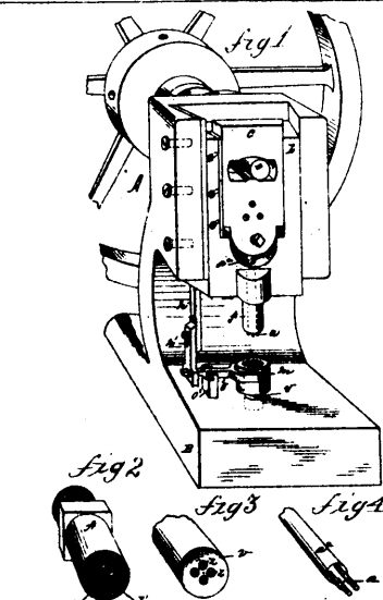
Merritt's Machinery and Process for Finishing Buttons.
