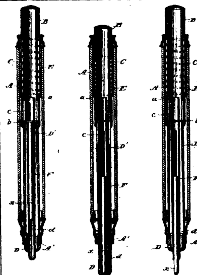
22164 Boman's Lead and Crayon Holder.
