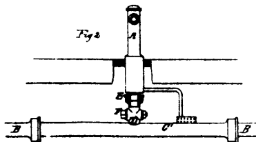
13263 Richards's Improvements on Ice Ploughs.
