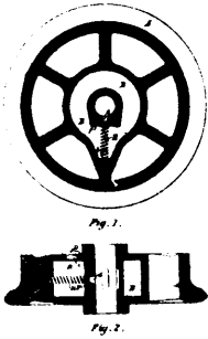
13253 Gaujot's Improvements on Self-lubricating Wheels.
