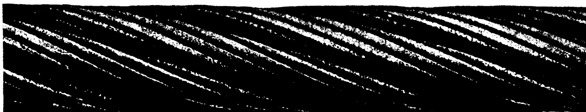
Illustration of Winding Rope, 240 fms. long x 3\frac{1}{2} circ. Galvanized Special Improved Patent Steel. Compound Make, supplied to Kennell Collieries, Bo'ness, Scot., which gave a record life of 6 years and 2 months. Showing condition when taken off.
