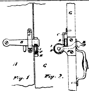
2255 Fraser's Door Latch.
