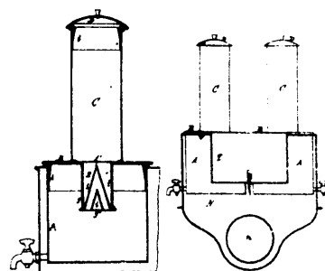
2262 Watkins & Tucker's Tea and Coffee Press
