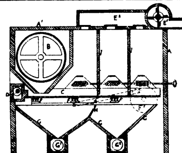
2258 Smith's Machine for Dressing Flour.
