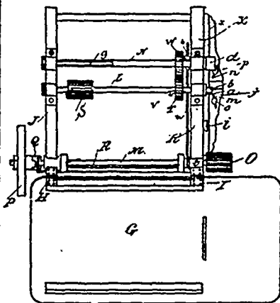
24213 Picard's Wood Working Machine.
