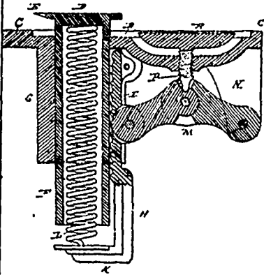
24207 Tyler's Bench Hook.
