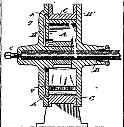
24215 Dowson's Engine for Steam or Water Power
