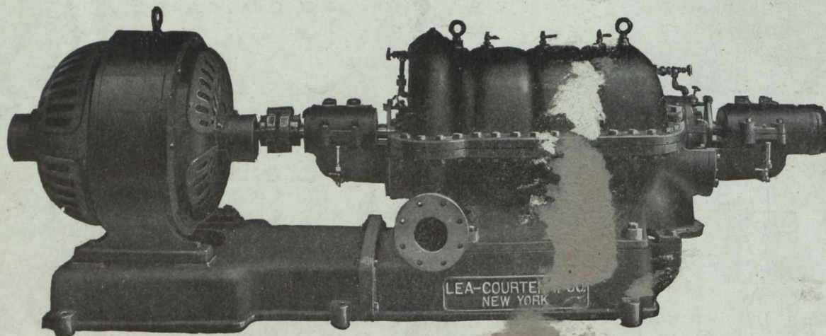
Lea-Courtenay 3-Stage Turbine Pump.
