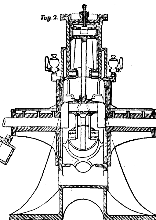
IMPROVED THREE-CYLINDER ENGINE.
