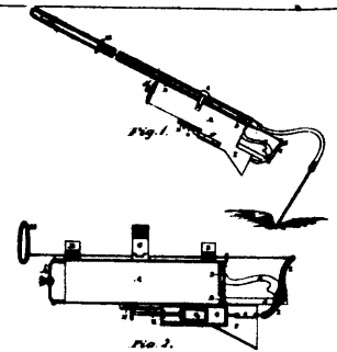
7418 Hyde & Elkins' Improvements on Hoes.
