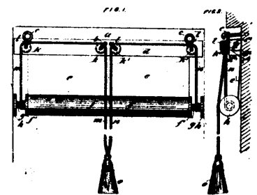
7424 Prévoet's Apparatus for Rolling and Unrolling Window Blinds.
