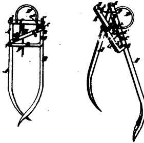
7411 Fisher's Improvements in Horse Hay Forks.
