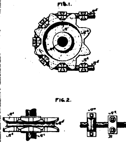
27311 Garland's Contrivance for Transmitting Power
