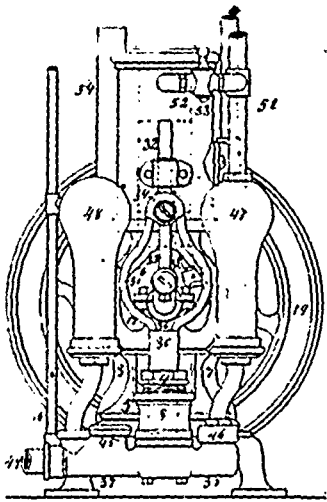
25025 Taylor & Hartig's Gas Engine Motor and Liquid Pump.
