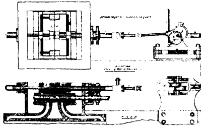
13520 Bain & Wallace's Improvements in Valve Gears.
