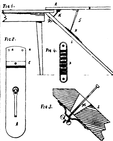
30958 Rideout's Ironing Board.
