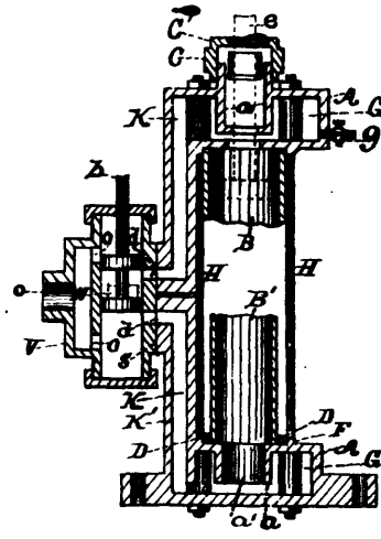
30960 Ross' Cylinder for Hydraulic Motors.
