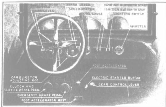
Illustration showing instrument Board on Chevrolet Four-Ninety. Electric starting and electric lighting switch, speedometer, electric horn, ammeter, oil indicator light equipment, gear shift lever. The Four-Ninety has selective sliding gear transmission with three speeds forward and reverse.
