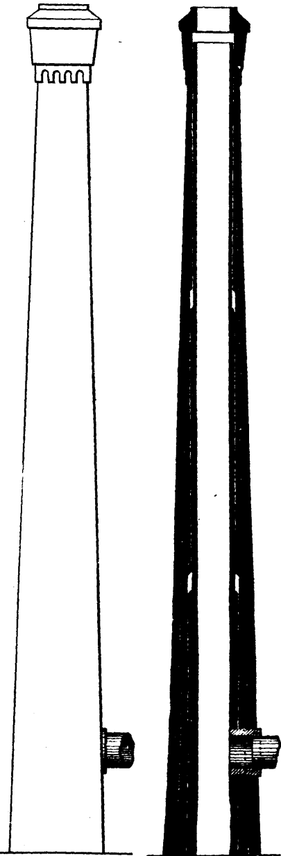
Figs. 2 and 3.—External View and Sectional Elevation of Chimney.
