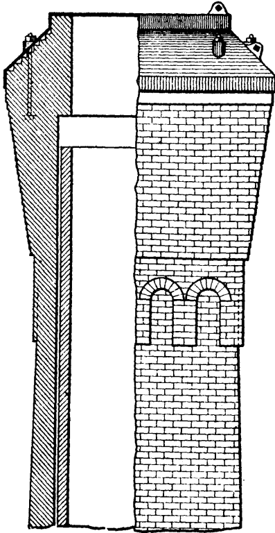
Fig. 1.—Finish for a Chimney Top.
