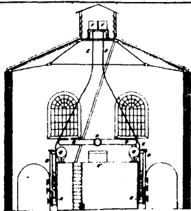
13317 Dixon's Improvements in the Manufacture of Gas.
