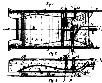
13313 Close's Improvements on Snow Clearing Machines.
