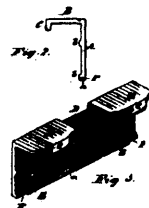
13319 Gives's Improvements on Saw Gauges.
