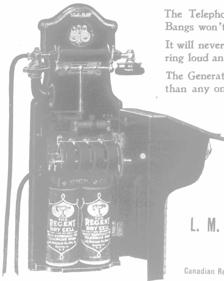
No. 522 Cradle Switch Type Equipped with 4-bar Generator and 160-ohm Ringer
