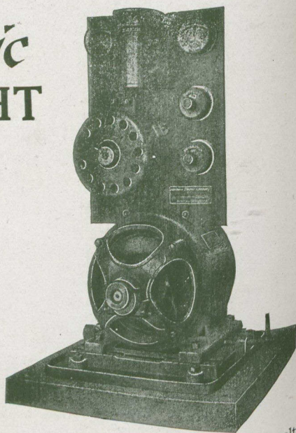
Northern Electric S-8 Belt-driven, 32 volt Electric Plant
