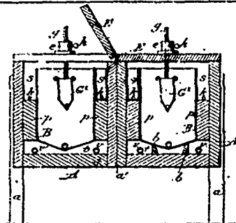
13648 Burrell's Improvements in Creamery Vats.
