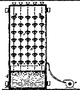
13638 Boomer &amp; Randall's Improvements on Vinegar Apparatus.
