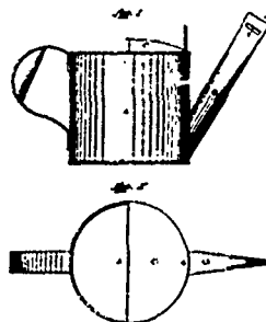
13642 Kemper's Improvements in Hand Seeders.
