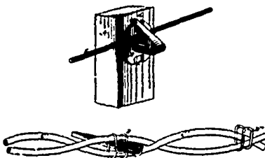
13641 Woodruff's Improvements on Fence Wire Fastenings.
