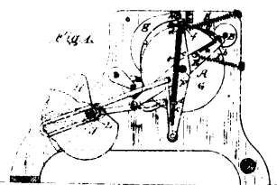
12113 Cross's Improvements in Paper Bag Machines.
