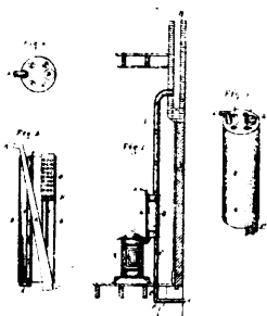
12108 Greenwood's Improvements in Air Heaters.
