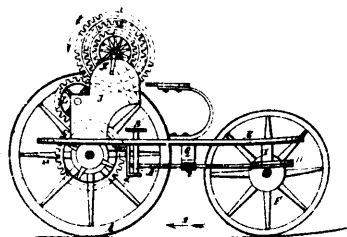
12119 Johnson's Improvements in Velocipedes.
