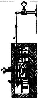
4081 Booth's Automatic Gas Light Extinguisher.
