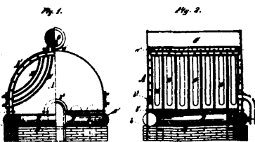
4090 Reashaw's Improvements on Steam Generators.
