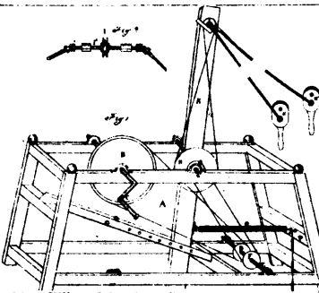
4764 Wilson &amp; Bowker's Machine for the Clipping of Horses and Sheep.
