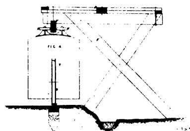
4766 Smith's Single Rail Railway.
